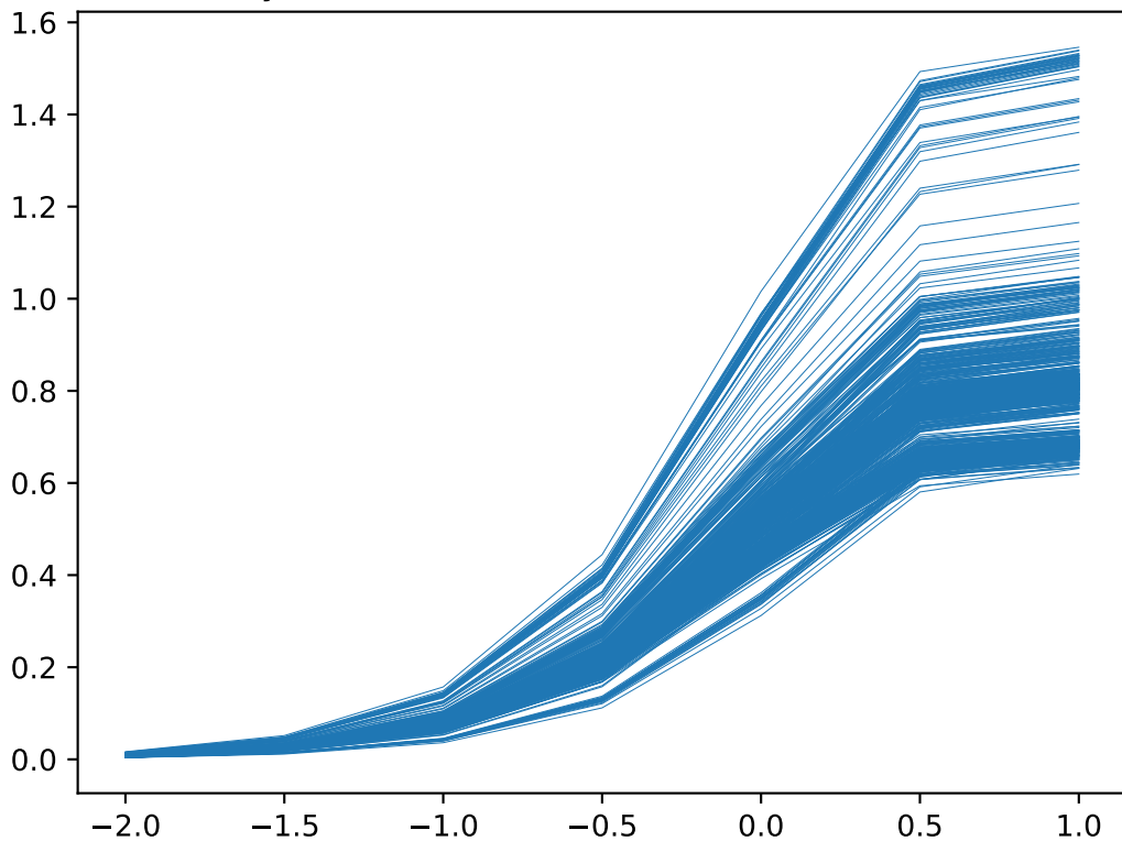
Dynamic Ricci Curvature for Geodesic 0.8
